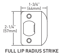
FULL LIP RADIUS STRIKE
